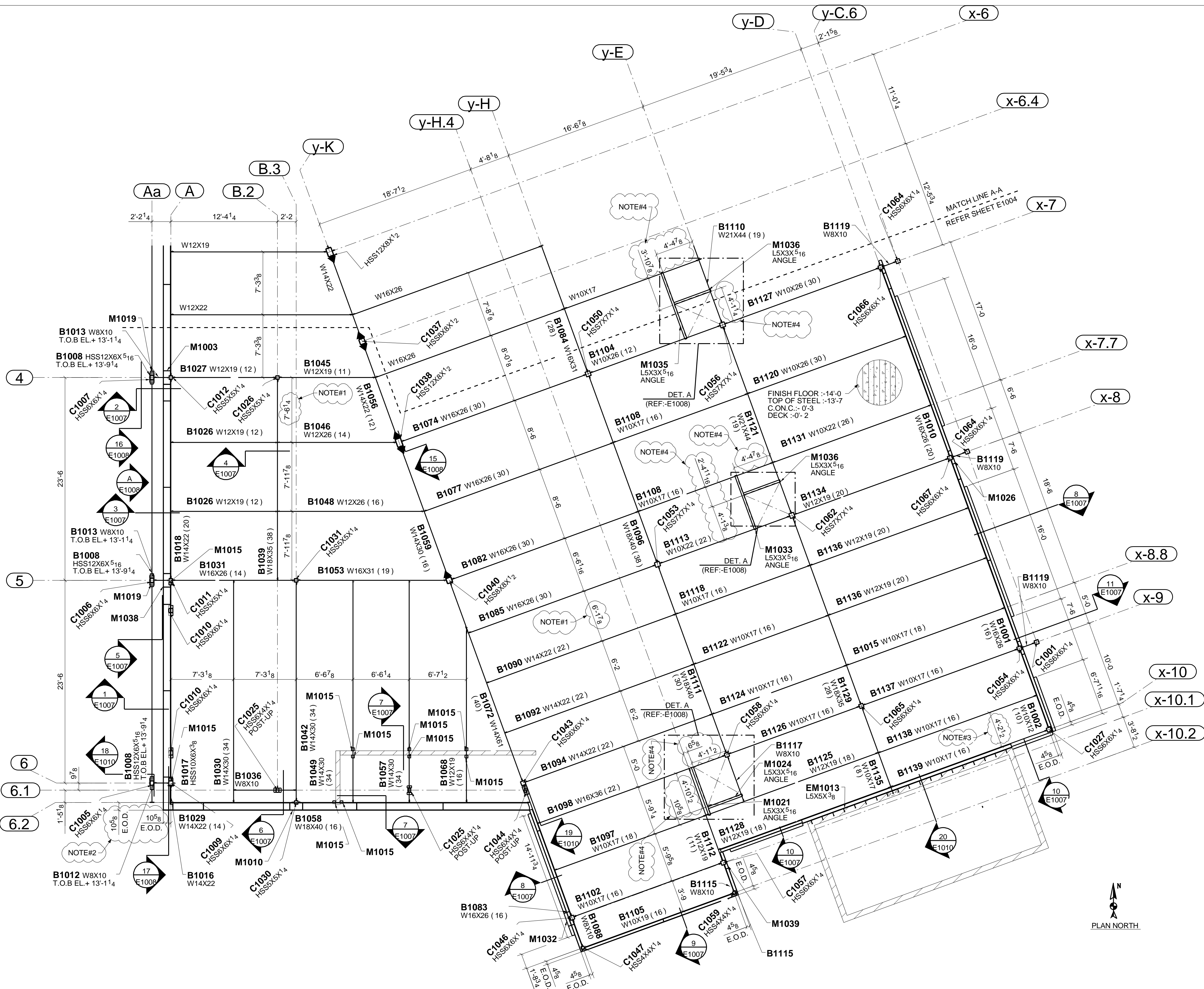
2ND FLOOR STEEL LAYOUT PLAN (T.O.S. EL.+13'-7") (UNO) (REF:-S1.03)
